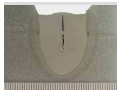
Weld depth to width ratio > 1 and relatively large amount of impurities in base material (S, P, Nb).
