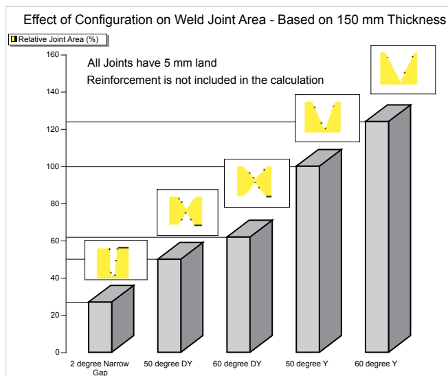
In 150 mm material thickness, 5 mm land - reinforcement not included.
